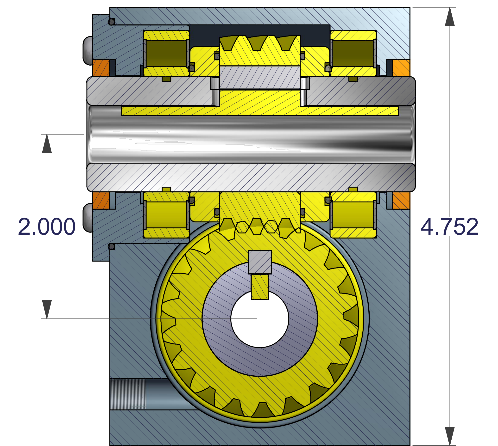
SECTION B-B SCALE 2
