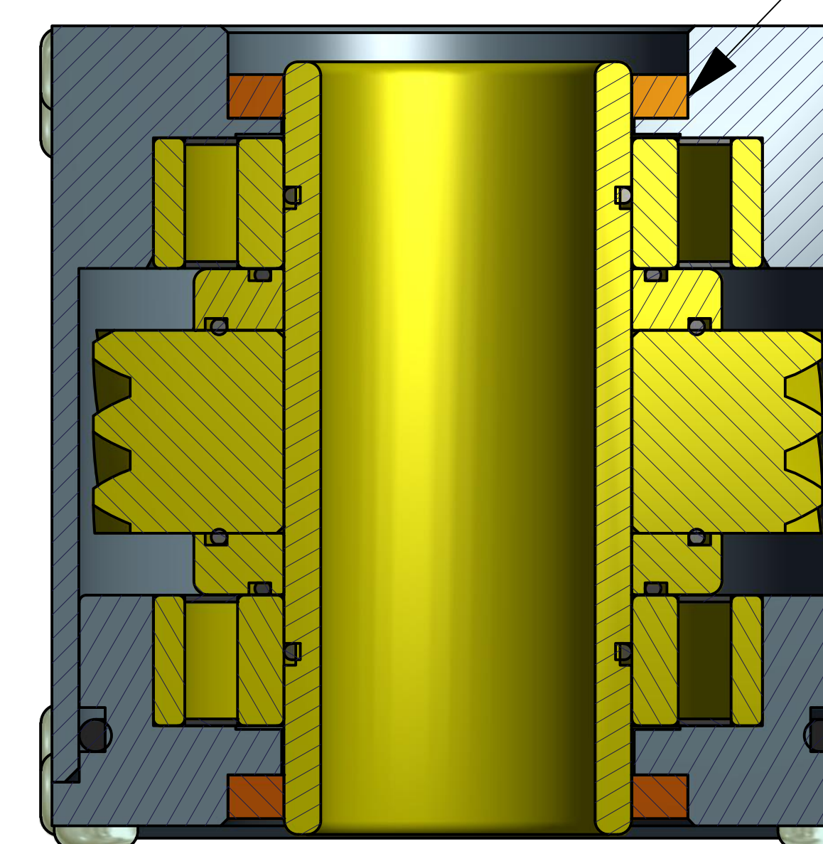
SECTION B-B SCALE 1.7
