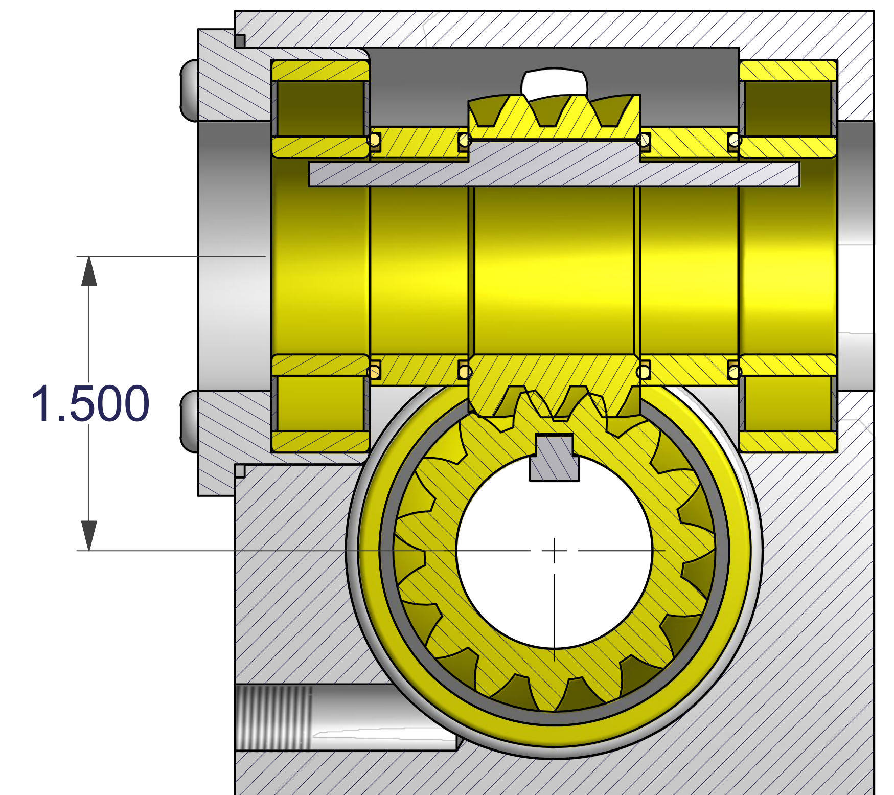
SECTION A-A SCALE 2
