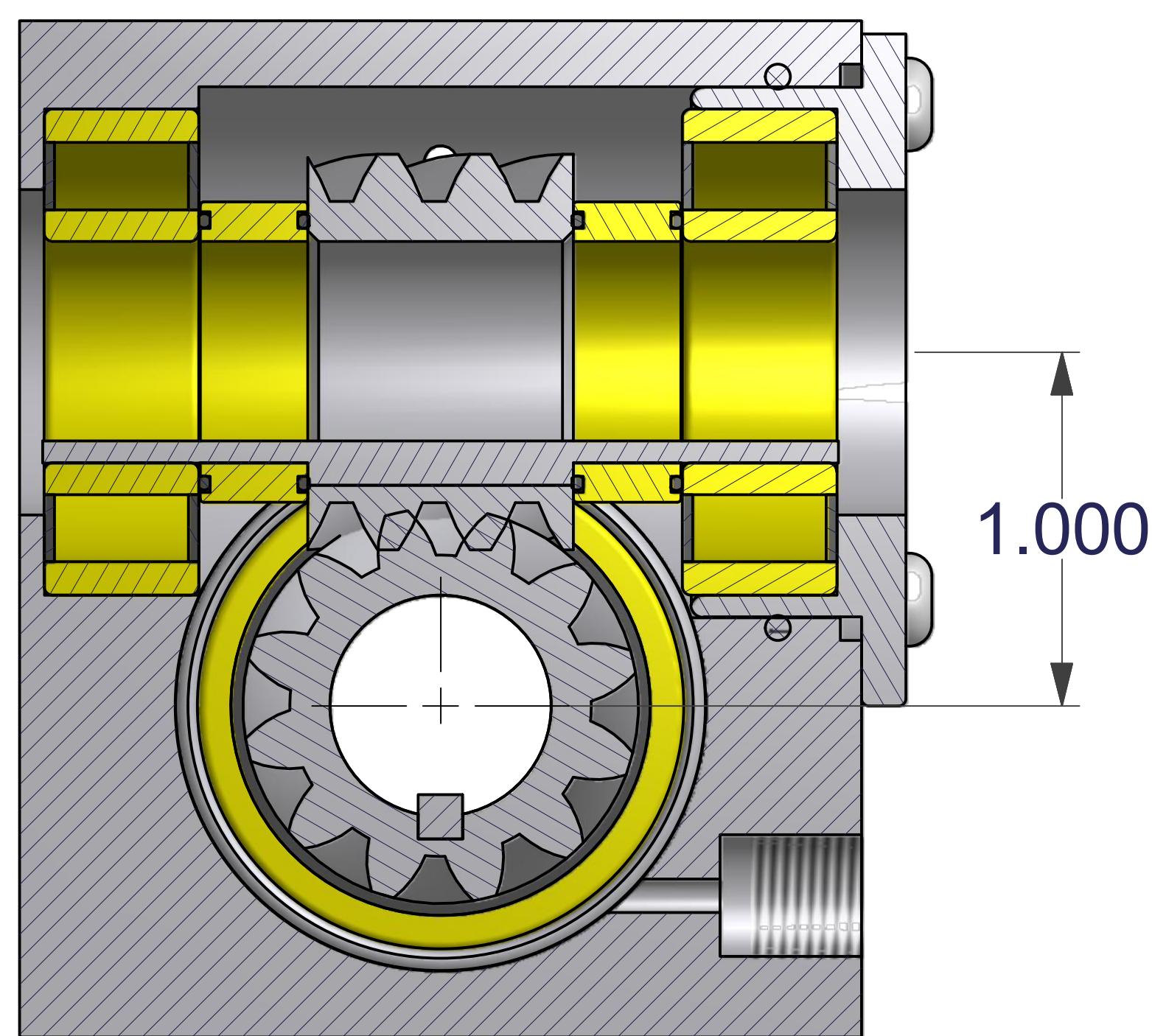
SECTION A-A SCALE 2.5
